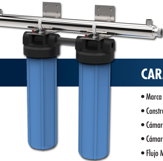
UV-50BB-2 WATER PURIFICATION SYSTEM
